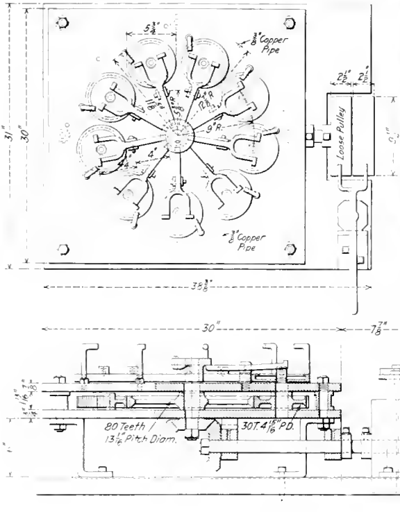
General Arrangement of Machine for Grinding Angle Cocks
